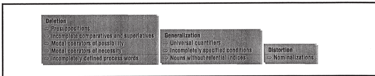
Figure 1. Linguistic defects.
